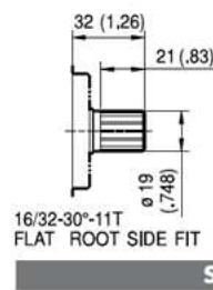
S2 16/32-30°-11T FLAT ROOT SIDE FIT Coppia Max Max Torque 230 Nm
