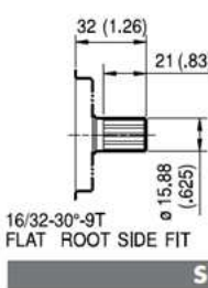
S1 16/32-30°-9T FLAT ROOT SIDE FIT Coppia Max Max Torque 110 Nm
